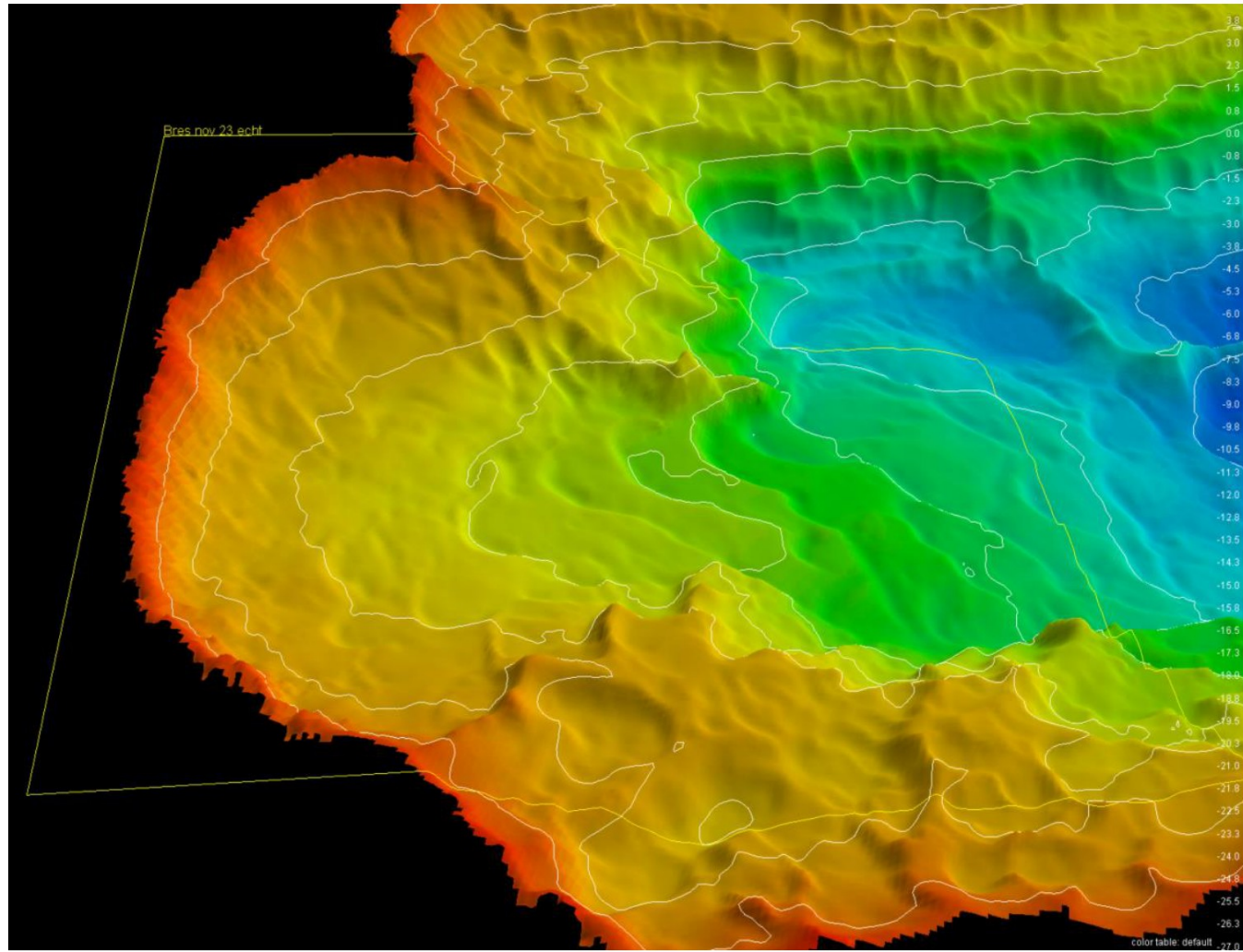
6.1 Peiling na bresval, 7-11-23
