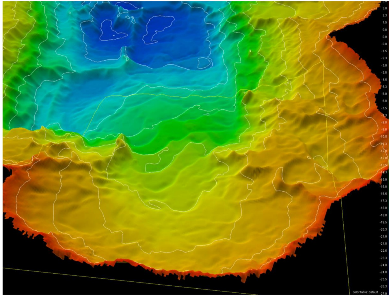
5.1 Peiling na bresval, 7-11-23
