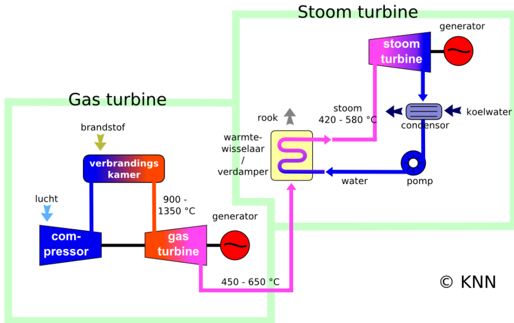
Figuur 4.4: Combined Cycle of STEG
